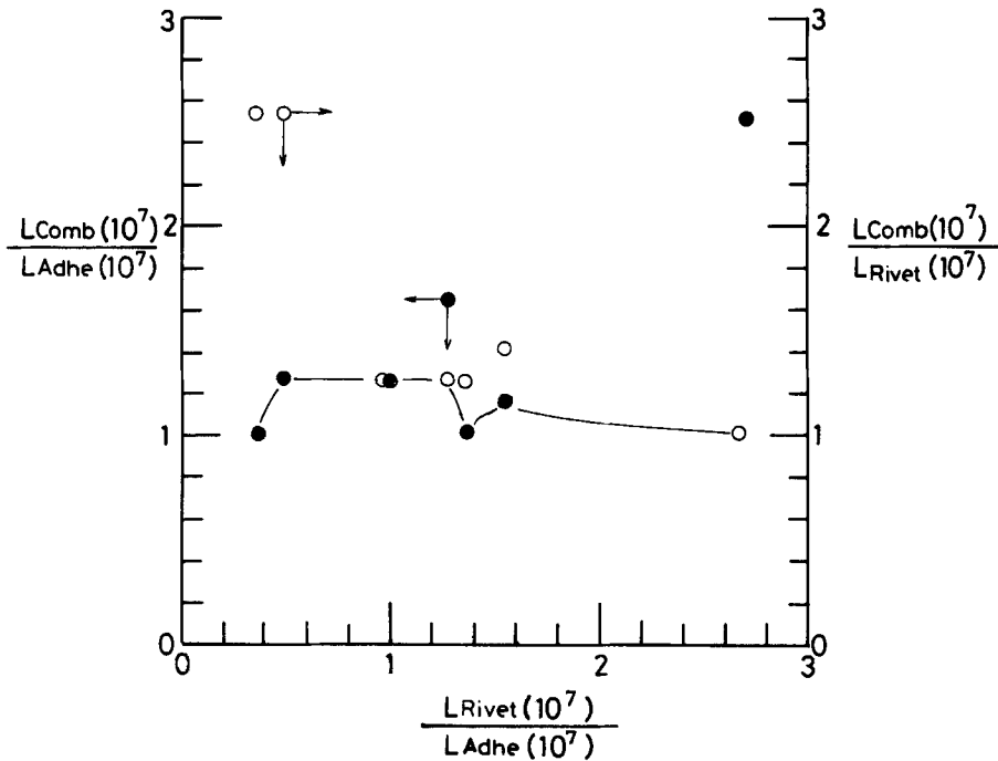
FIGURE 6 Effect of fatigue strength ratio of rivet joint to adhesive joint on the degree of increase in fatigue strength through combination.
