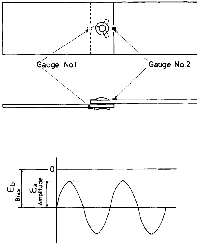
FIGURE 3 Bonding positions of strain gauges and schematic illustration of output wave.
